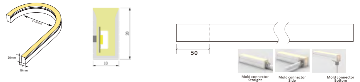
24V DC Side Bend 10*20mm Neon flex
