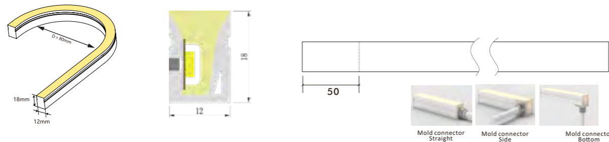
24V DC Side Bend 12*18mm Neon flex
