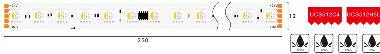
24V DC 4 Pixel 5 Line 12mm 5050 96LED RGBW Color 4pixels Dmx Strip
