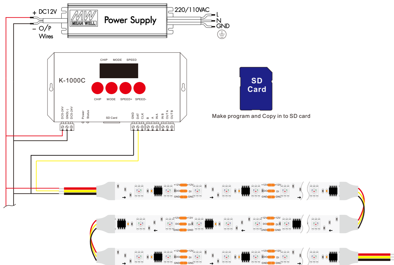
Programmable controller
