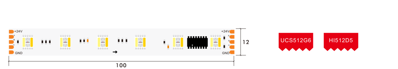
24V DC 10 Pixel 5 Line 12mm 5050 60LED RGBWW Color 10pixels Dmx Strip
