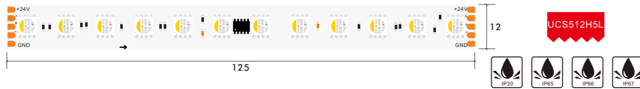
24V DC 8 Pixel 5 Line 12mm 5050 96LED RGBW Color 8pixels Dmx Strip
